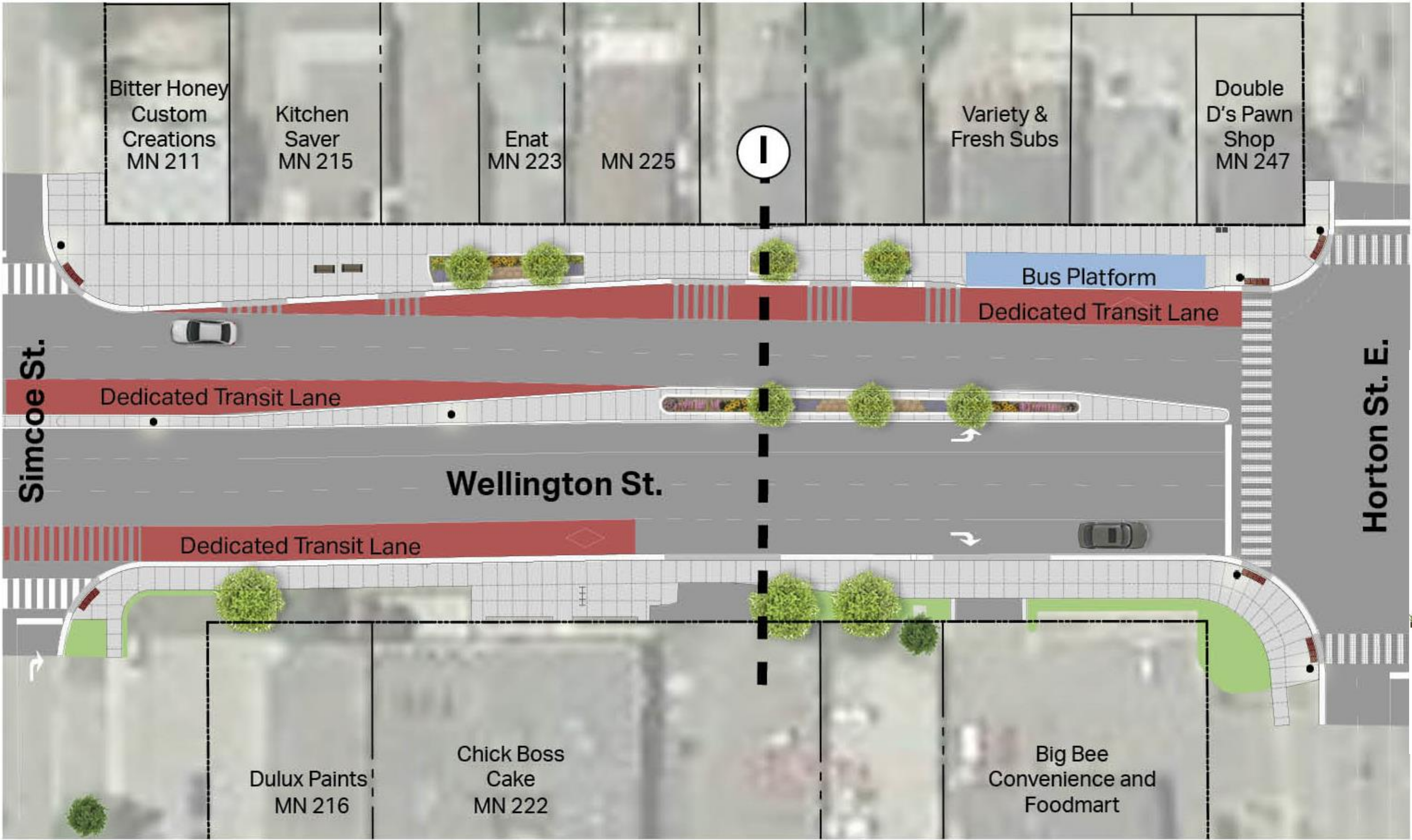
Wellington Street -- Section I
