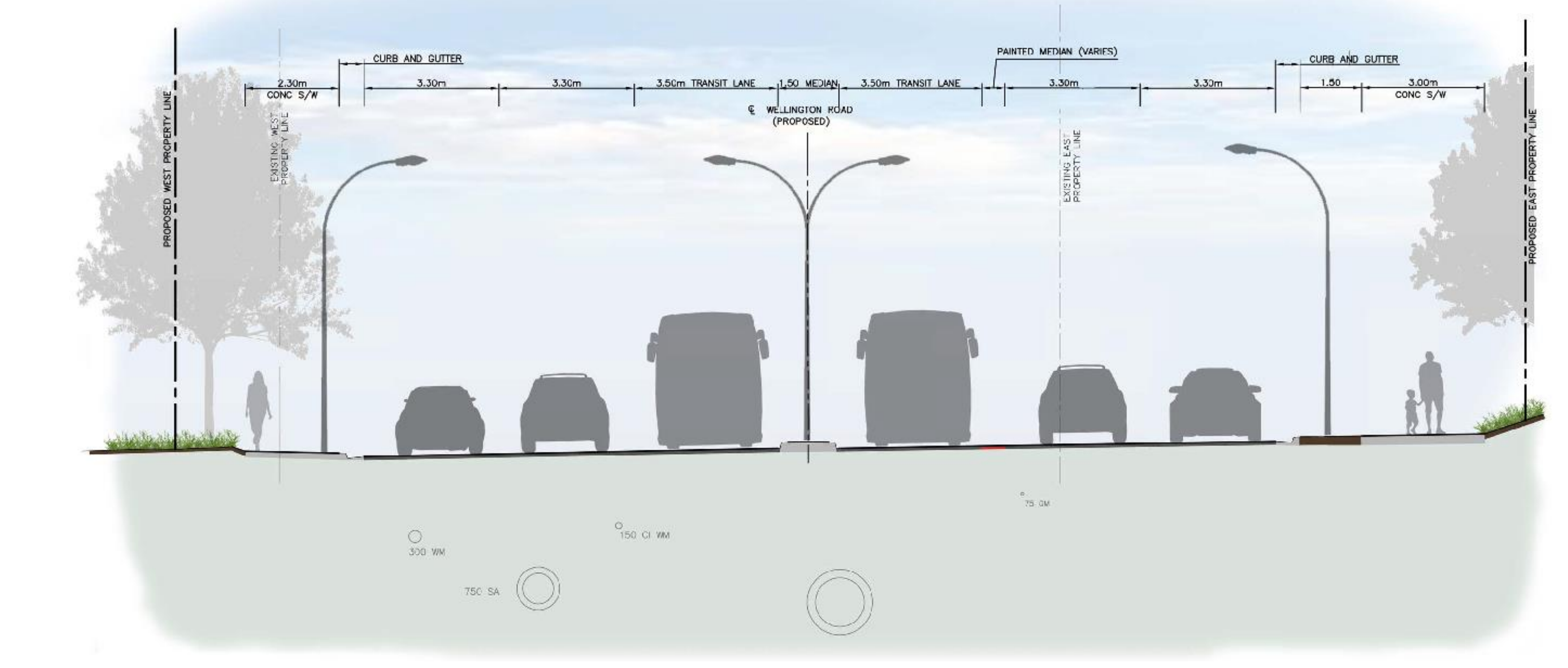
B Wellington Road – Section B
