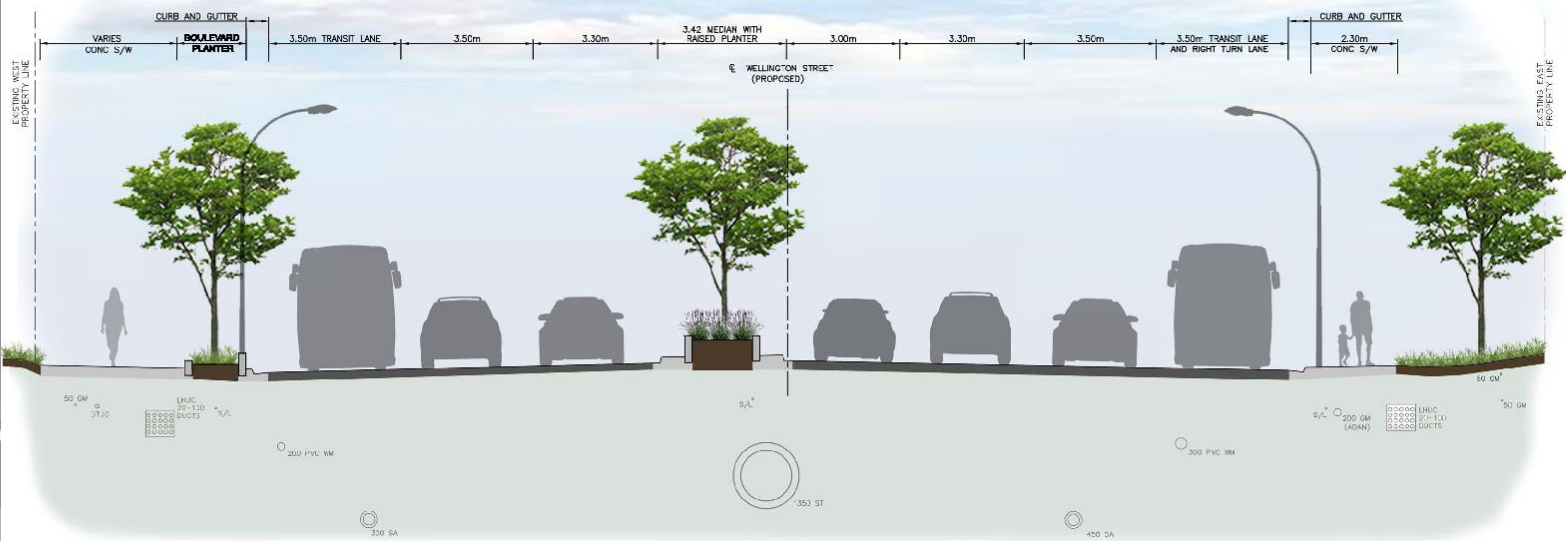
Wellington Street -- Section I
