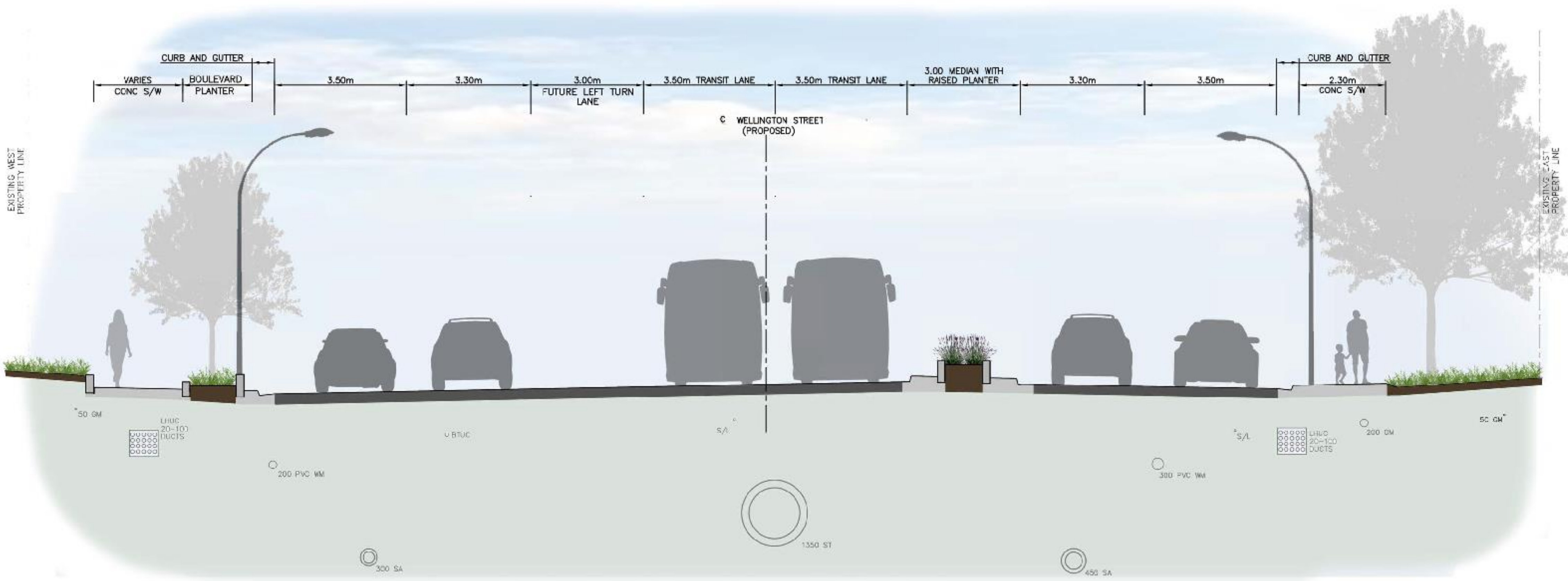
H Wellington Street – Section H
