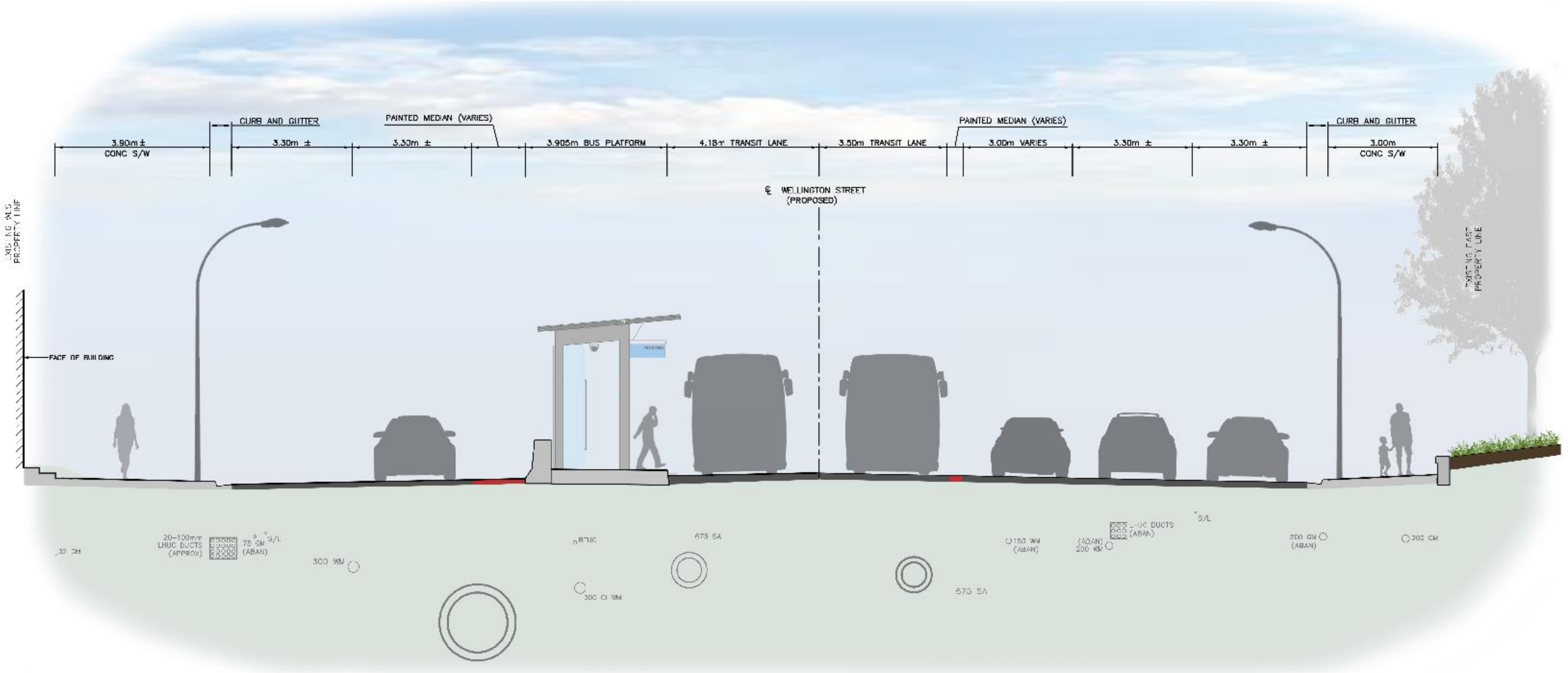
E Wellington Street- Section E
