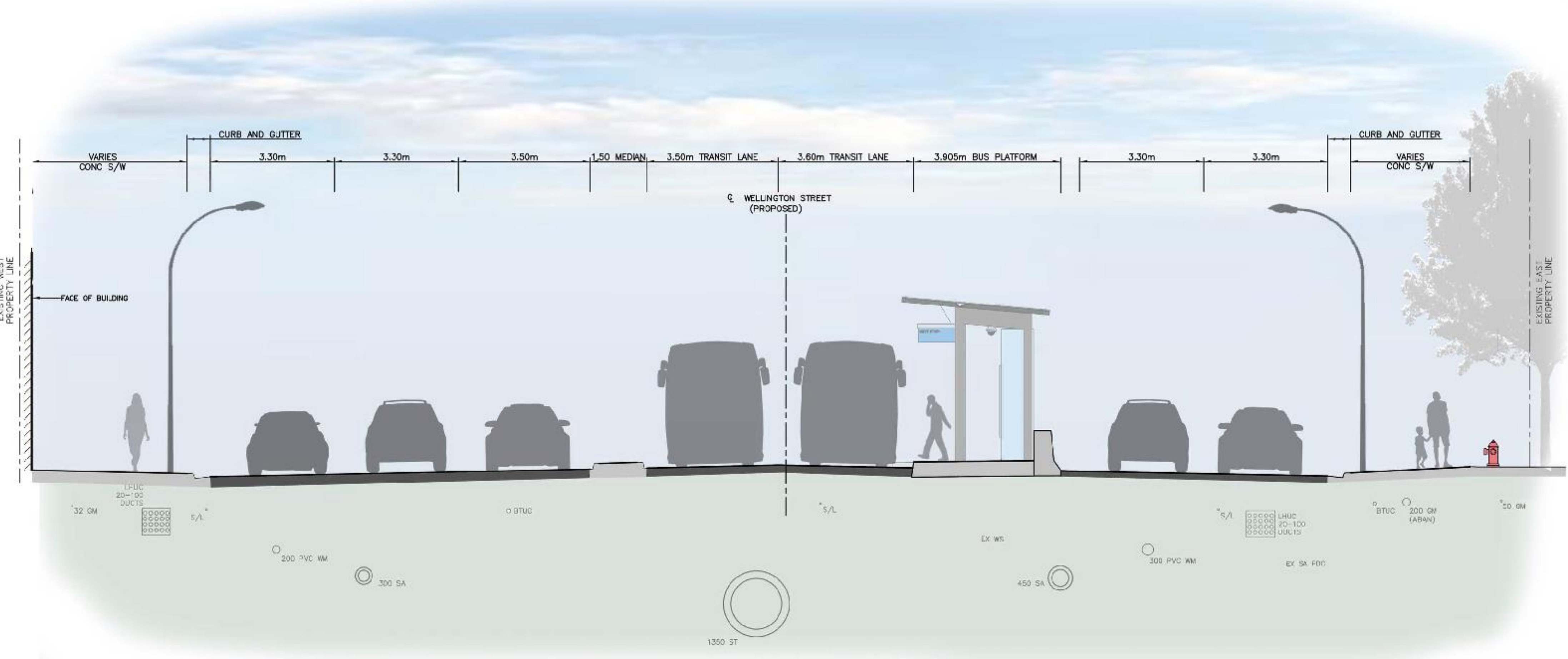
F Wellington Street -- Section F
