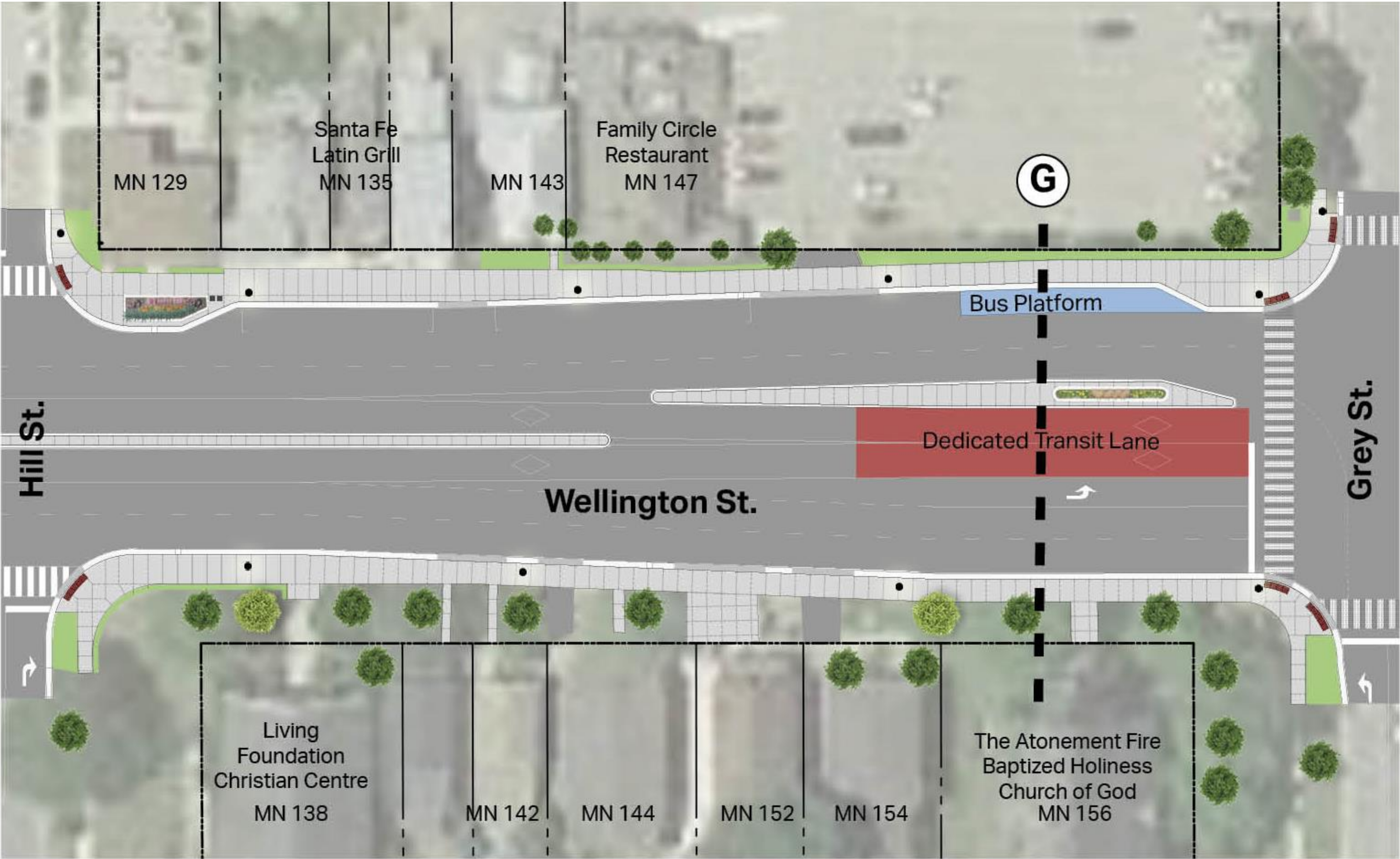
G Wellington Street – Section G
