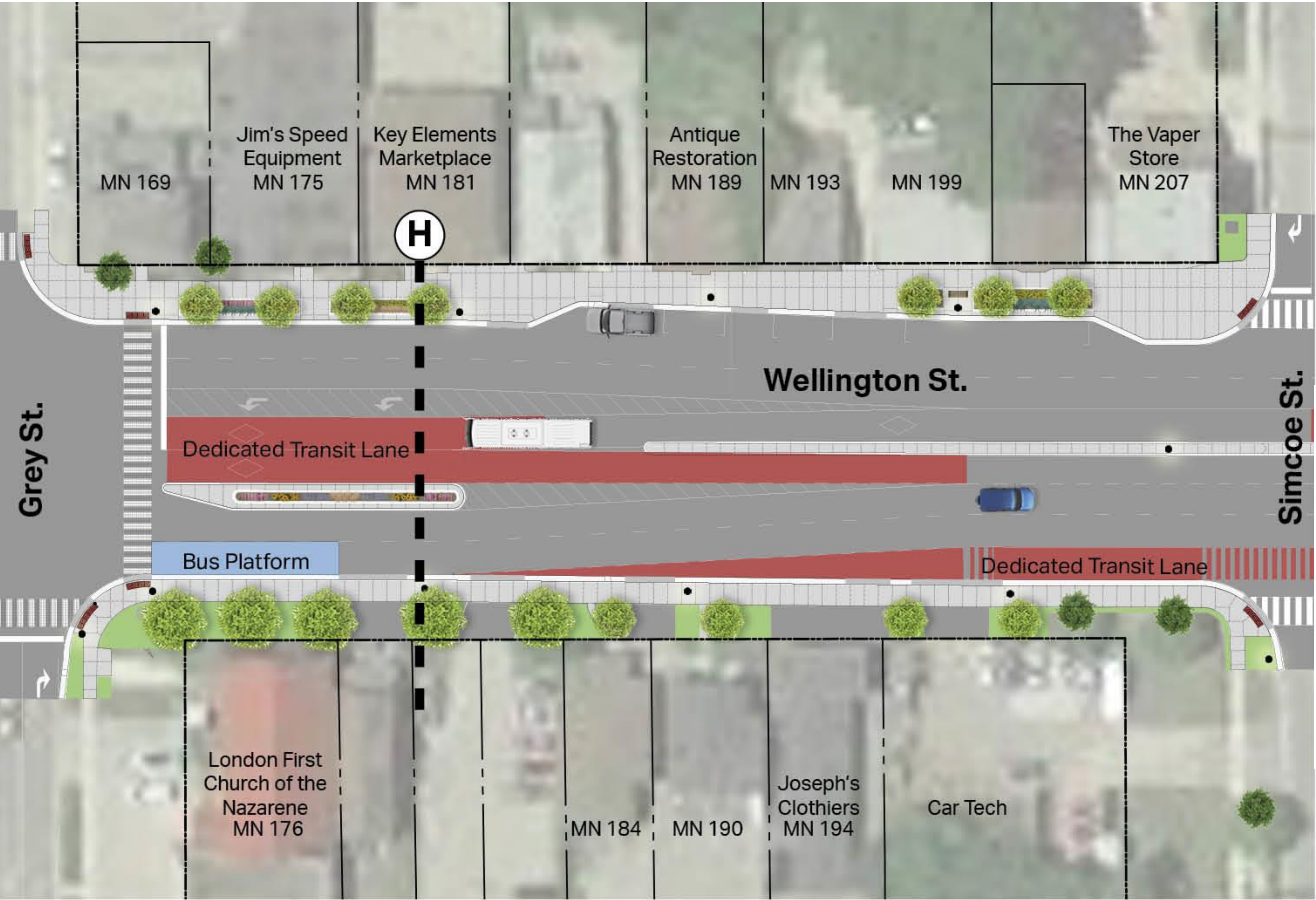
H Wellington Street – Section H
