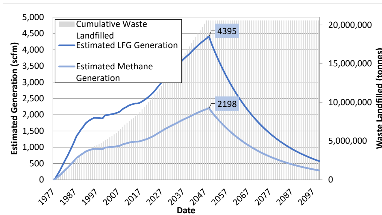
Figure 5: Estimated Total Landfill Gas and Methane Generation for the W12A Landfill Expansion
