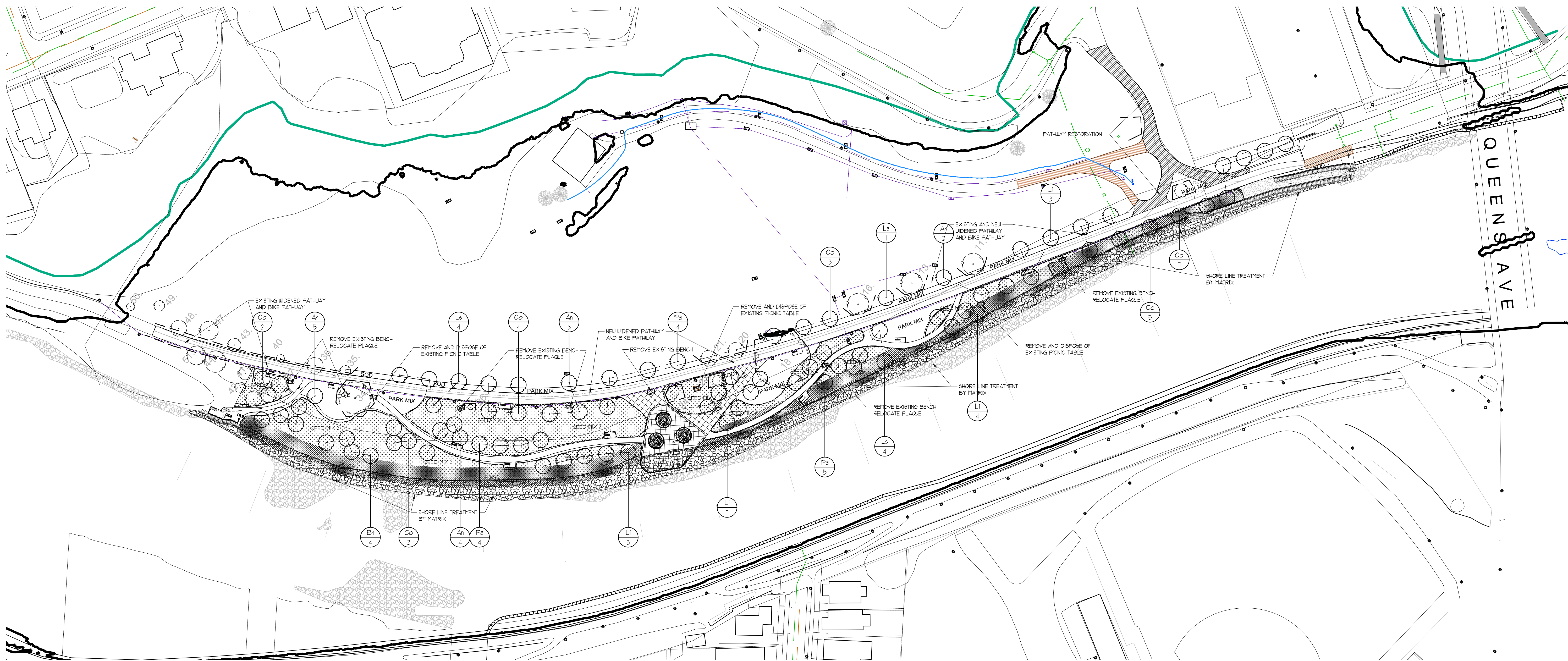
LANDSCAPE PLAN SCALE = 1:750M
