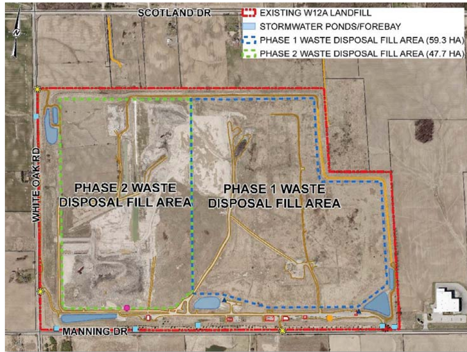
Figure 3 - W12A Landfill
