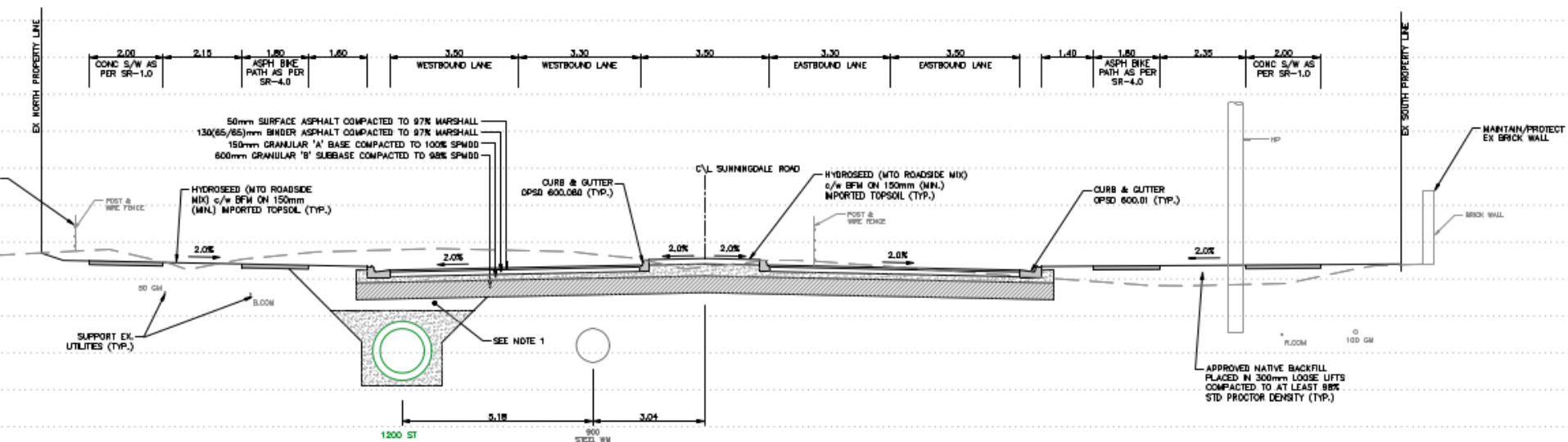
SUNNINGDALE ROAD - STATION 1+400
