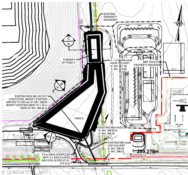
SCALE 1:1,500 m
