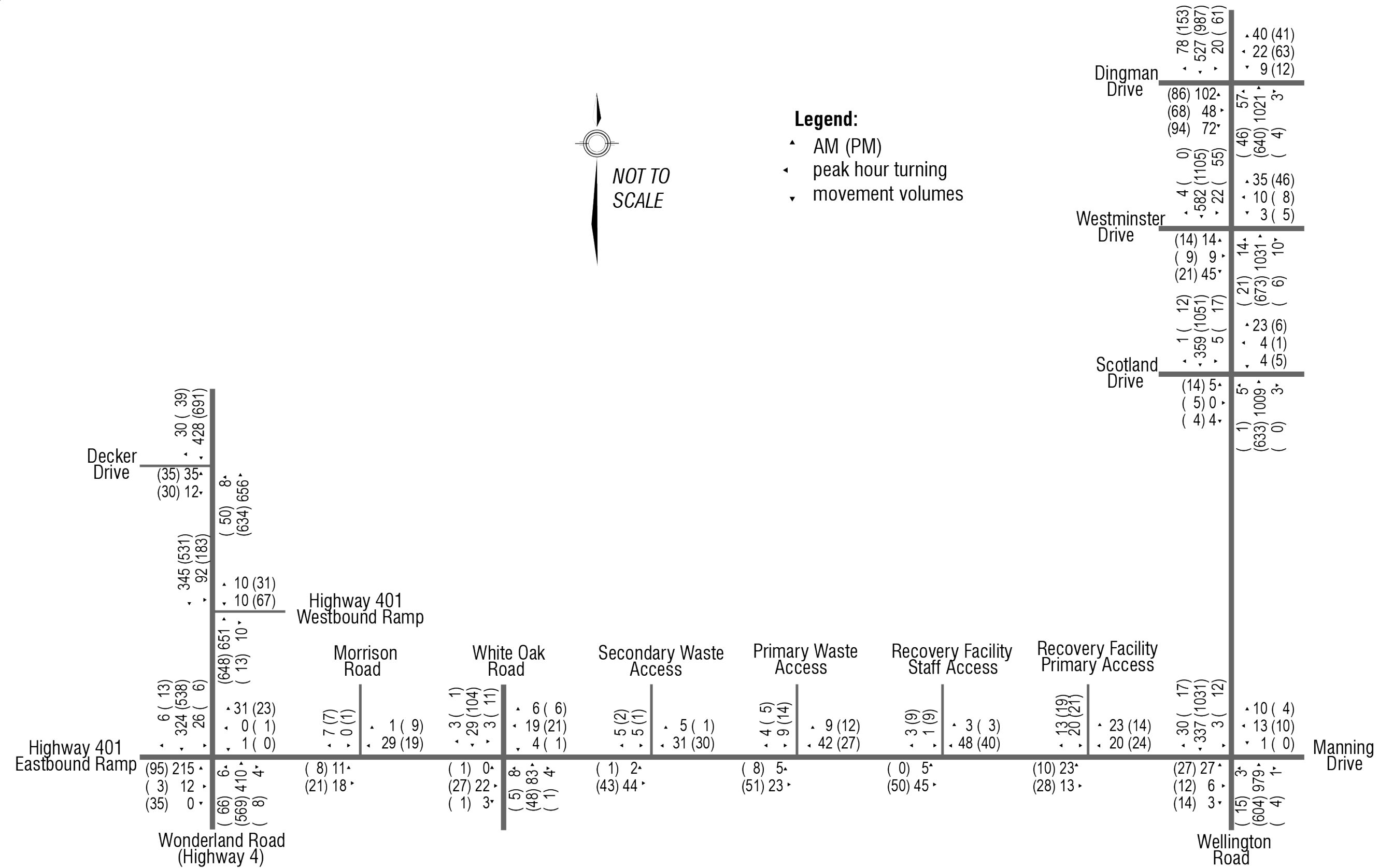
Figure 6: Future (2048) Traffic Volumes
