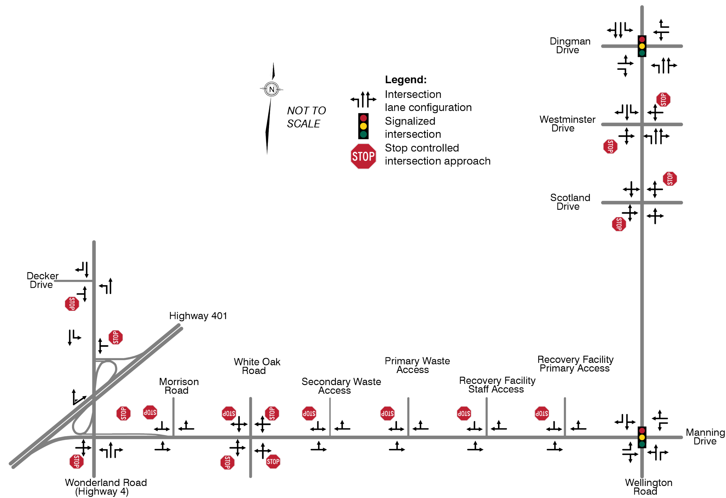
Figure 2: Lane and Traffic Configurations
