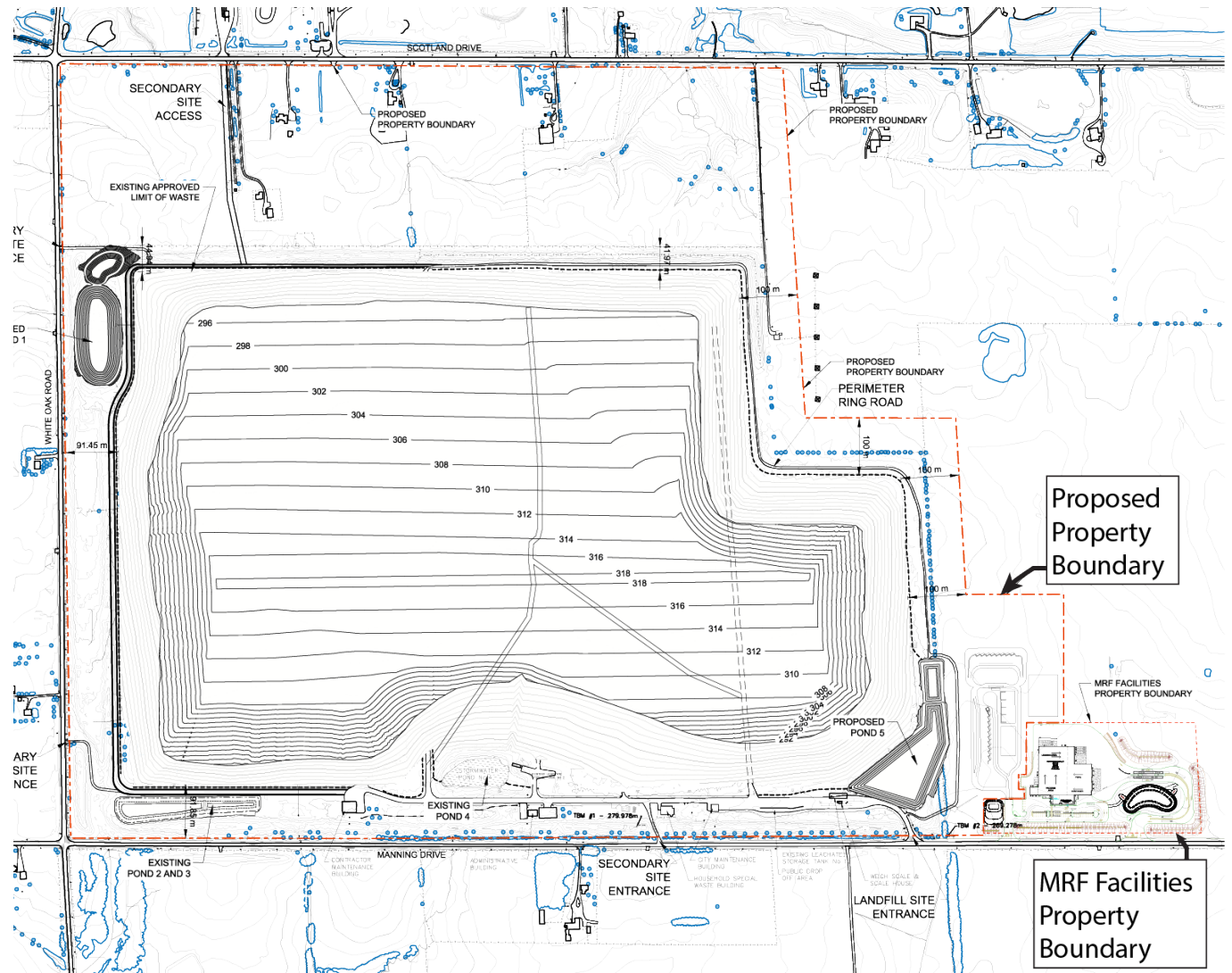
Figure 4: Conceptual Expansion Plan
