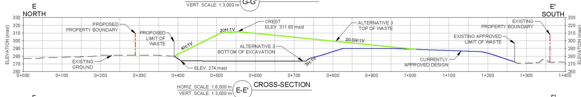
CROSS-SECTION G-G'
