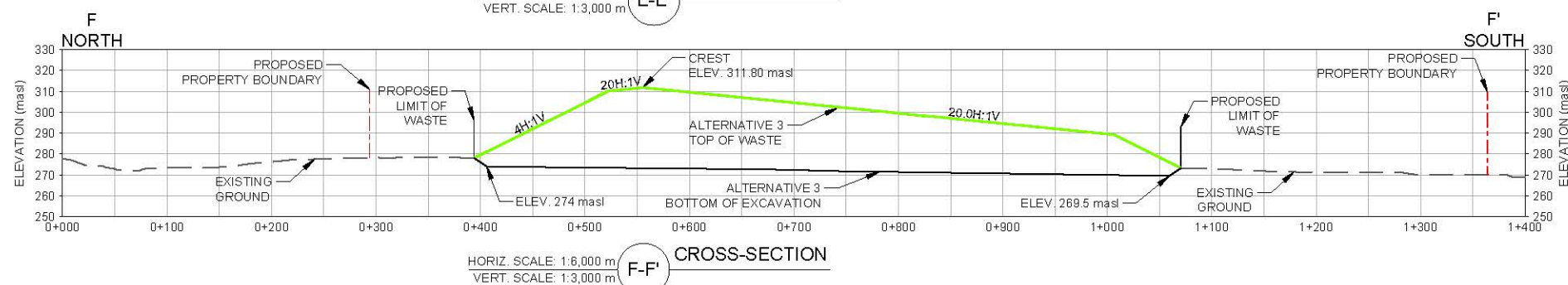
CROSS-SECTION E-E'
