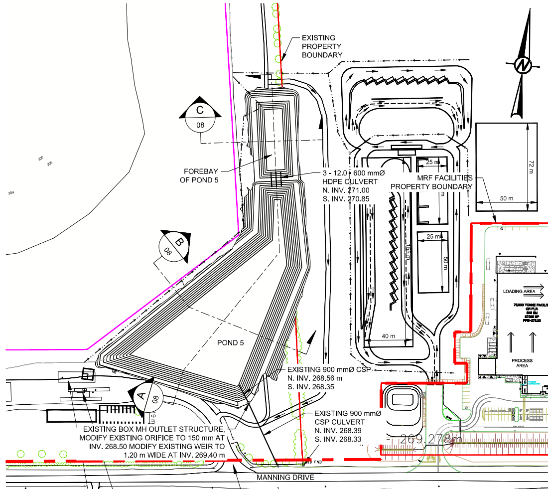
PLAN VIEW OF POND 5 AND FOREBAY SCALE 1:1,500 m
