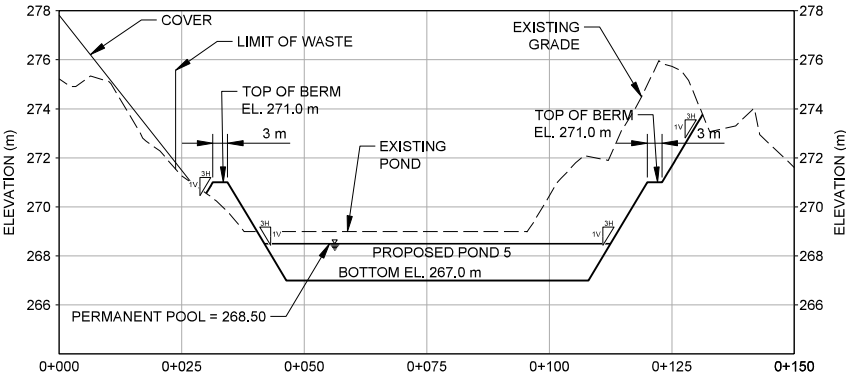
CROSS-SECTION SCALE 1:750 m V.E.=x5
