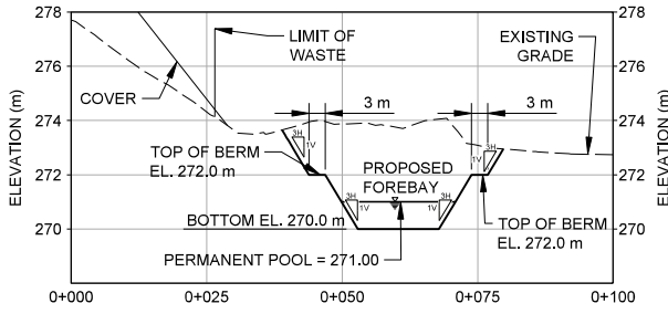
CROSS-SECTION SCALE 1:750 m V.E.=x5
