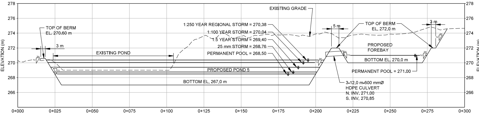
SECTION SCALE 1:750 m V.E.=x5
